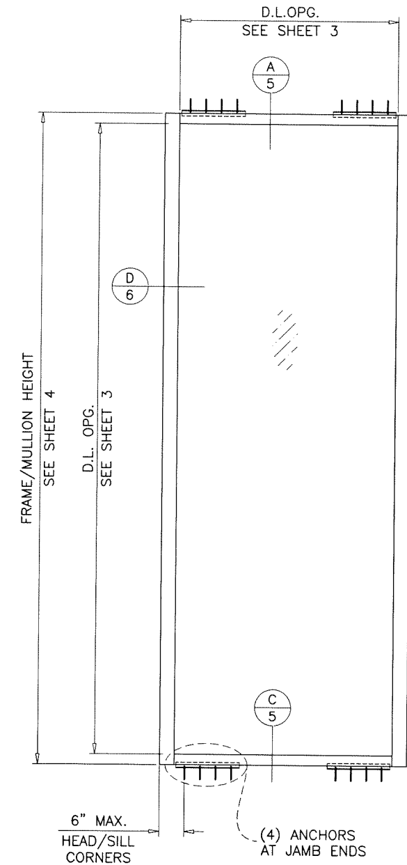
SINGLE 'O' PANEL: FRAME WIDTH = D.L.O. WIDTH + 7.00" FRAME HEIGHT = D.L.O. HEIGHT + 5.00"
