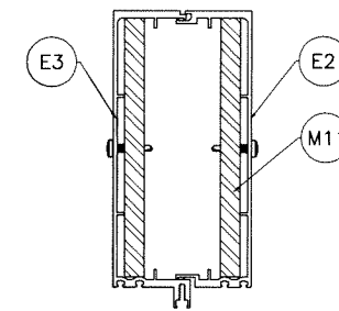
MULLION 'DM'
